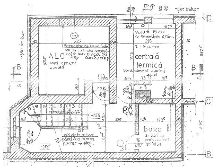
PLAN SUBSOL -250
