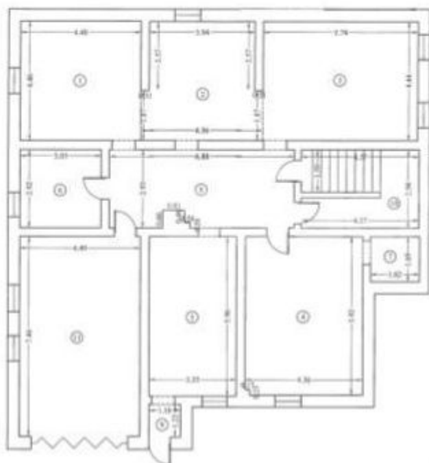
PLAN SUBSOL
