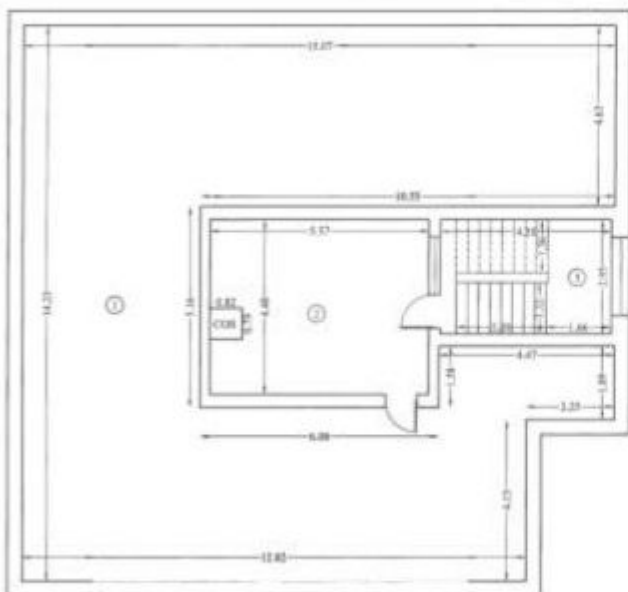
PLAN MANSARDA
